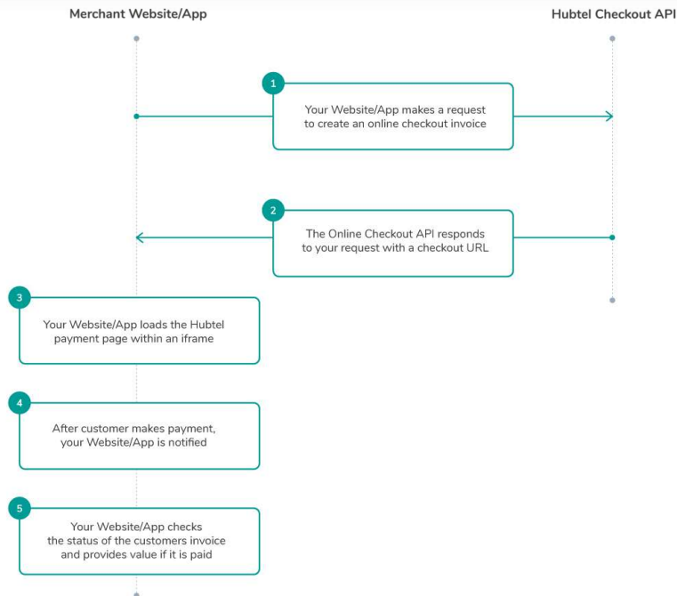
Onsite Checkout Request Flow
