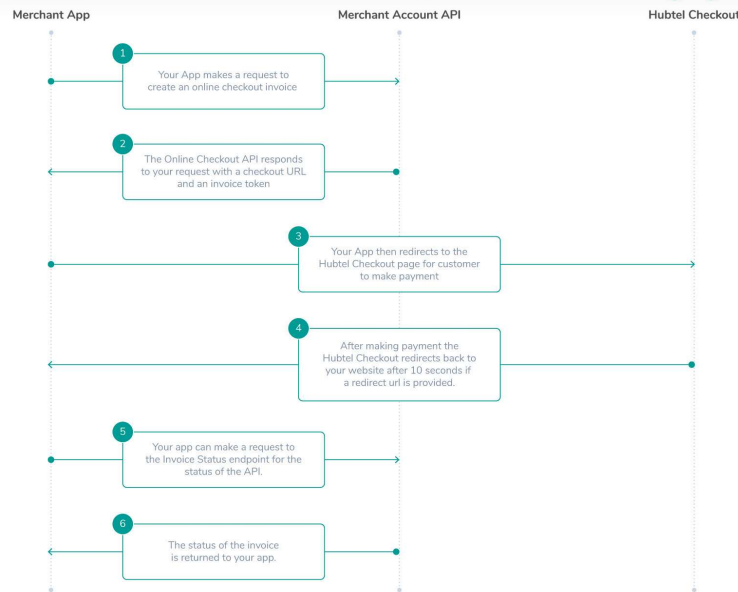
Redirect Checkout Request Flow
